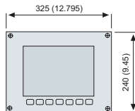
10,4" LCD Monitor (color)
