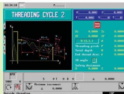
Threading
