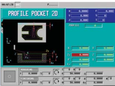
Pockets with 2D profile
