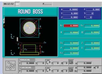
Rectangular and circular boss
