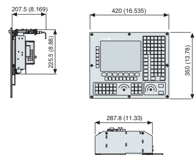
Central Unit - Monitor (color and monochrome) - Keyboard
