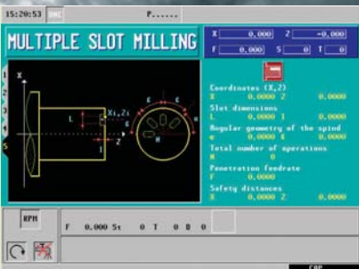
Multiple slot milling
