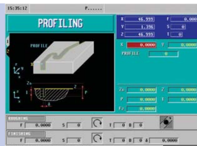
Profile milling
