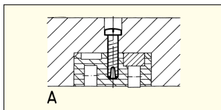
Self tapping screw
