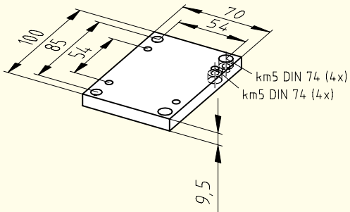
Figure 9: Adapter plate AP-70-02
