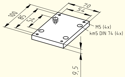
Figure 10: Adapter plate AP-70-03
