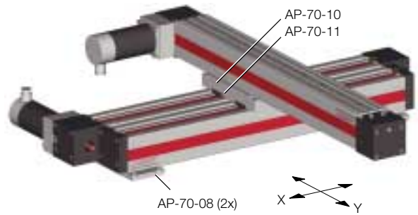
Figure 6: Boom system
