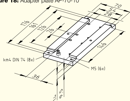
Figure 18: Adapter plate AP-70-10
