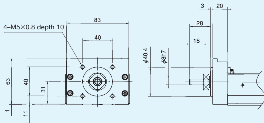
Fig. 16 KR46 Housing A without motor flange (Specification □ □ 60)
