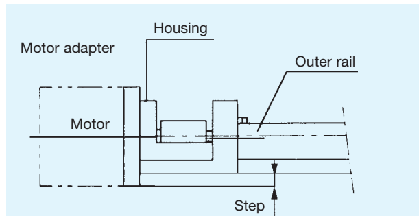
Fig. 19 Motor-Connection
