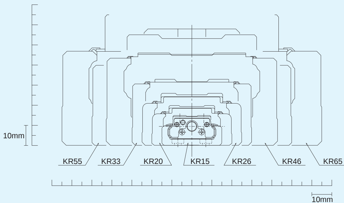
Fig. 6 Cross-Sectional View
