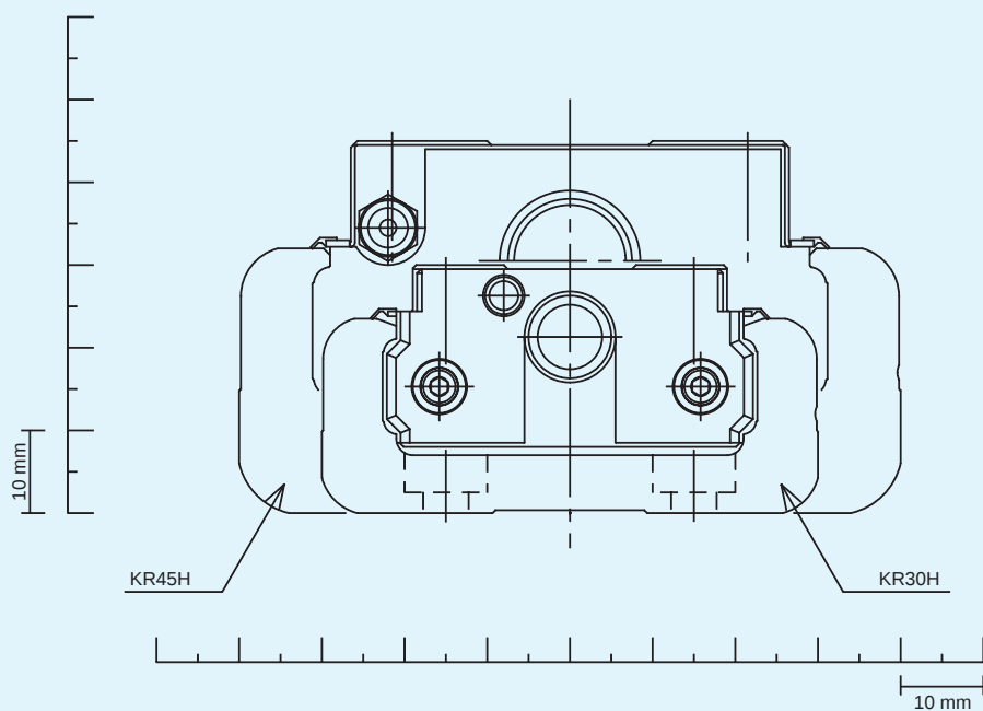
Fig.7 Cross-Sectional View
