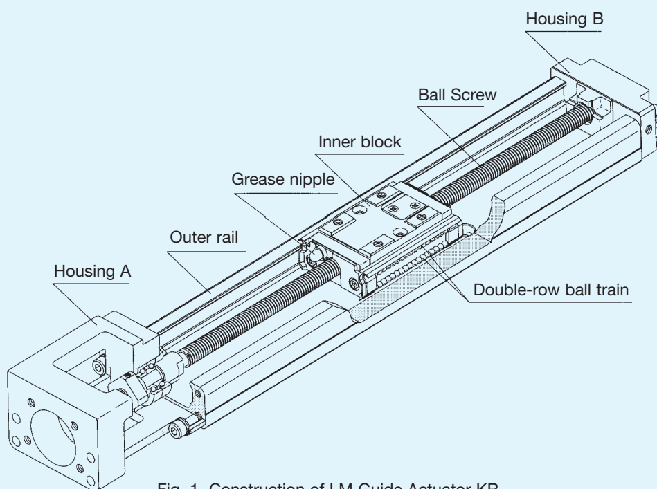
Fig. 1 Construction of LM Guide Actuator KR
