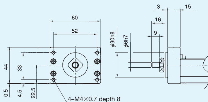
Fig. 13 KR33 Housing A without motor flange (Specification 30)
