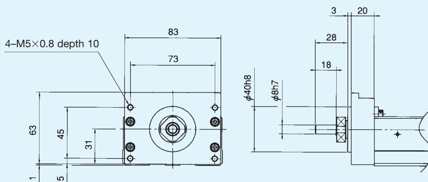
Fig. 15 KR46 Housing A without motor flange (Specification 50)
