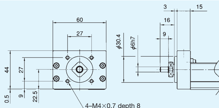
Fig. 14 KR33 Housing A without motor flange (Specification 40)
