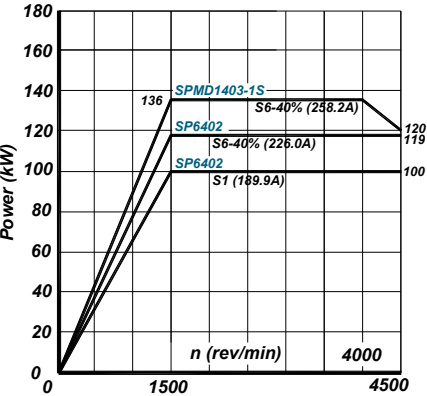
Power/speed and torque/speed graphs for S1 and S6-40% cycles. FM9-B113-C5Cx-E01 with CT drives.
