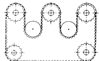
Multi-shaft drive
